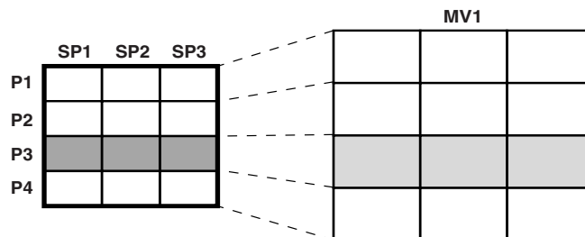
Figure 15–1 Determining PCT Freshness
