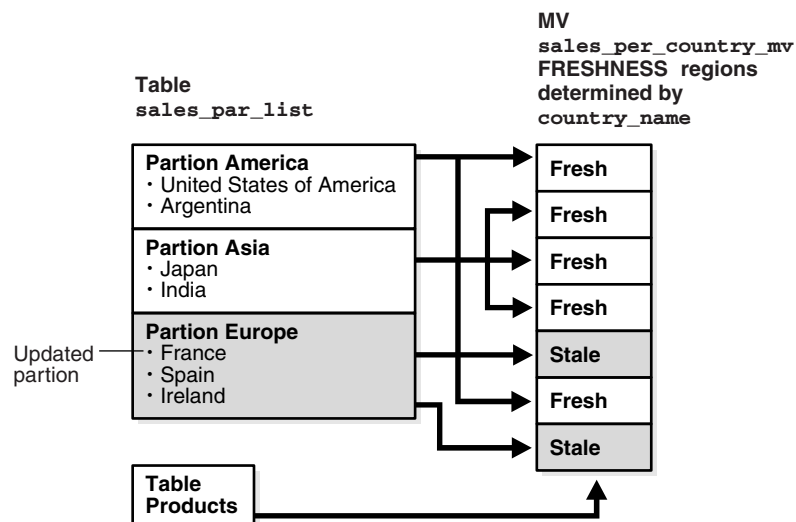
Figure 18–4 PCT Rewrite and List Partitioning
