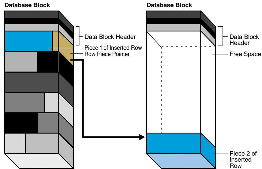
Figure 12-14 Row Chaining
