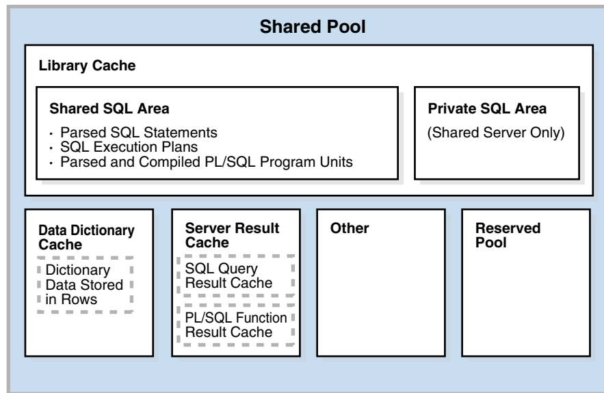
Figure 14–8 Shared Pool
