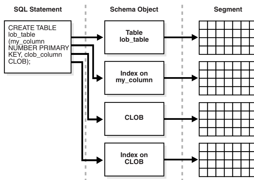
Figure 12–19 Multiple Segments
