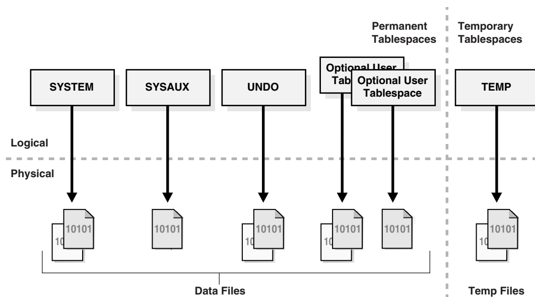
Figure 12-23 Tablespaces
