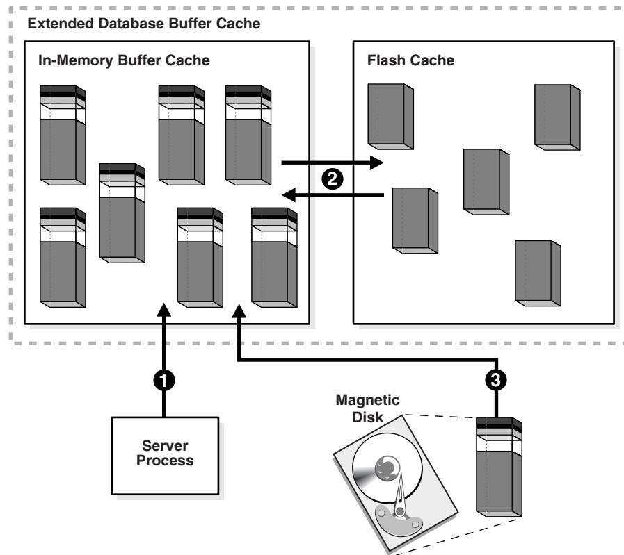
Figure 14–5 Buffer Search
