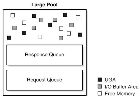
Figure 14–10 Large Pool
