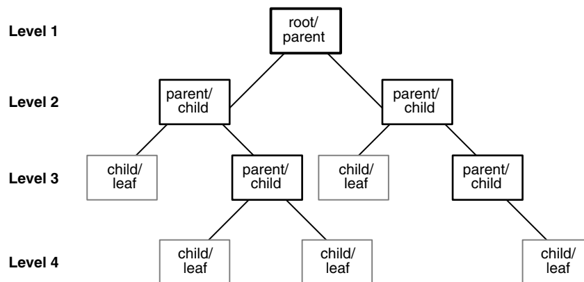
Figure 2–1 Hierarchical Tree
