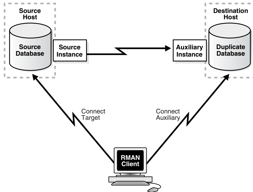
Figure 23–2 Active Database Duplication
