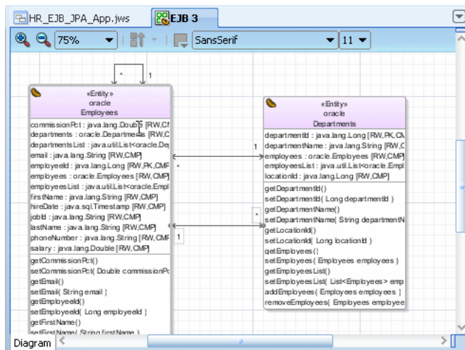
Figure 7-2 Persistence Model
