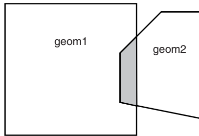
Figure 24–3 SDO_GEOM.SDO_INTERSECTION
